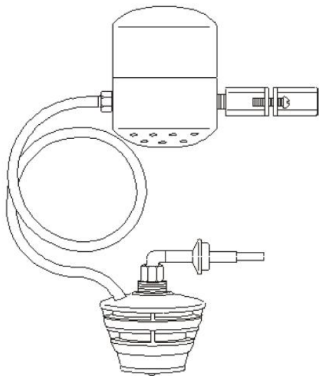
Chamber pod self-evacuation design drawing
